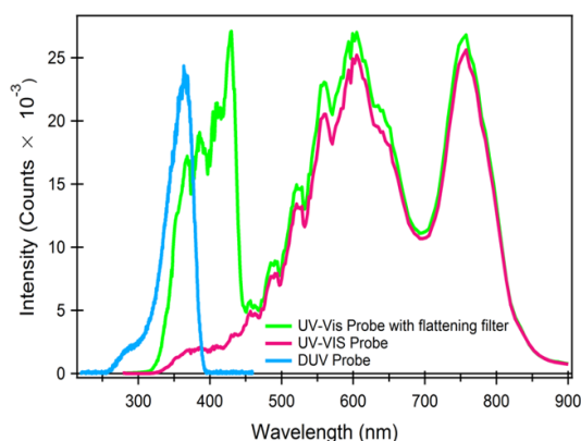
Figure 3. DUV and UV-Vis continuum used for probing. The UV-Vis spectrum after the flattening filter is also shown.
